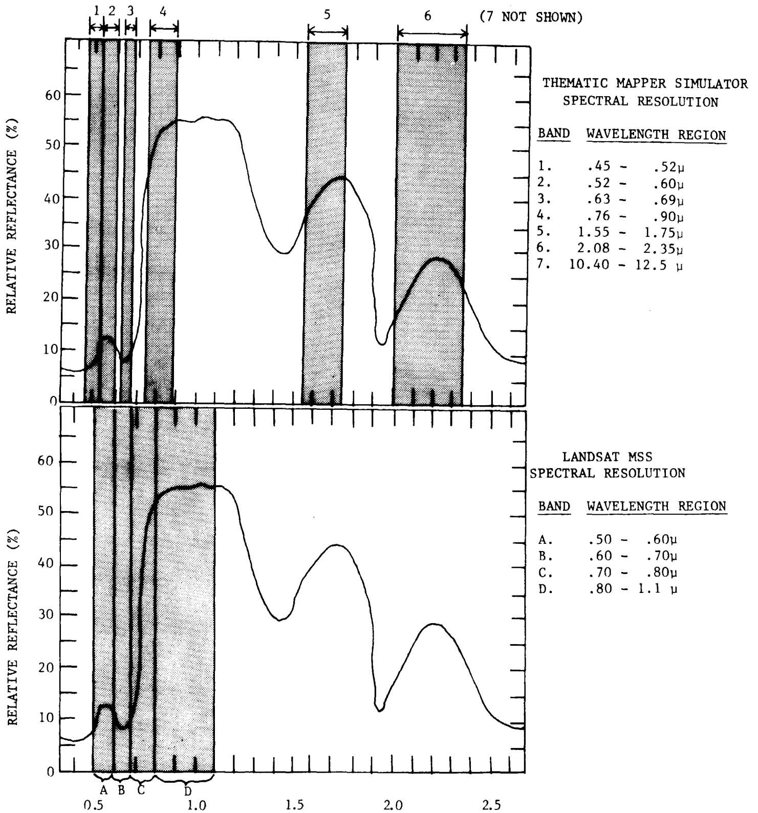
Figure 1. Spectral Wavelength Characteristics of TMS and Landsat MSS Systems
